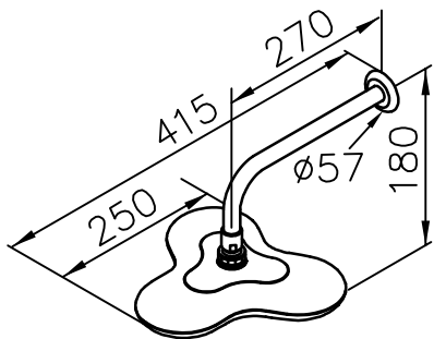
Rain Shower (Without Diverting Function)
