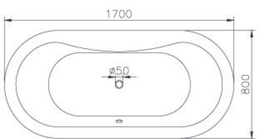
0360-D0-7900 Bathtub 1700*800*480mm
